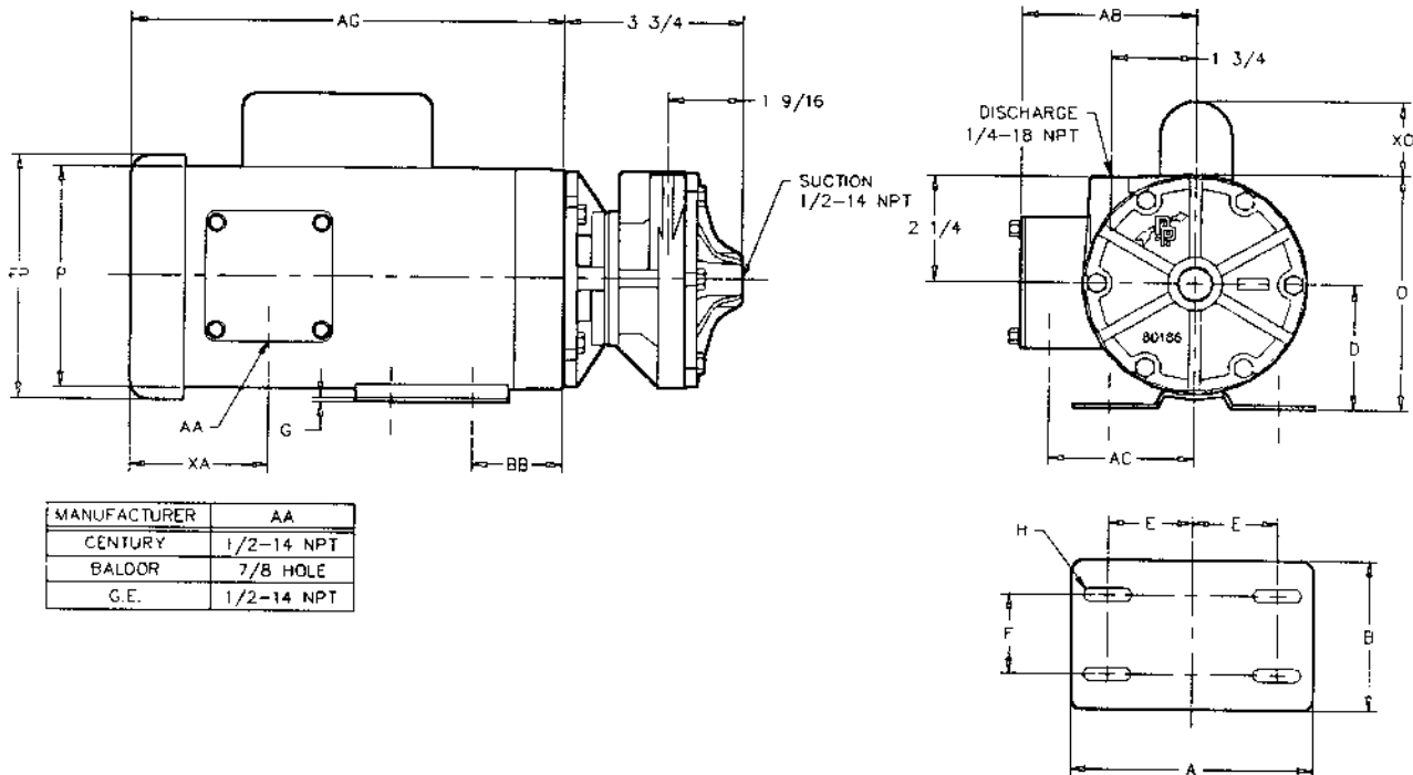
MOTOR FRAME DIMENSIONS
